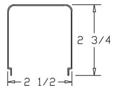
RIBBED DIFFUSER
