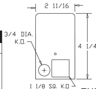
END W/O PLATE
