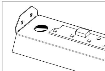
SELF BENDING TABS FOR ATTACHING COVER
